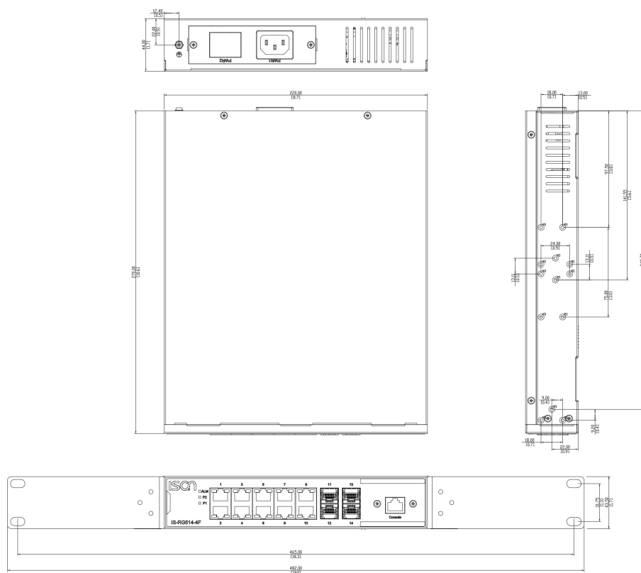
(Single Mounting)
