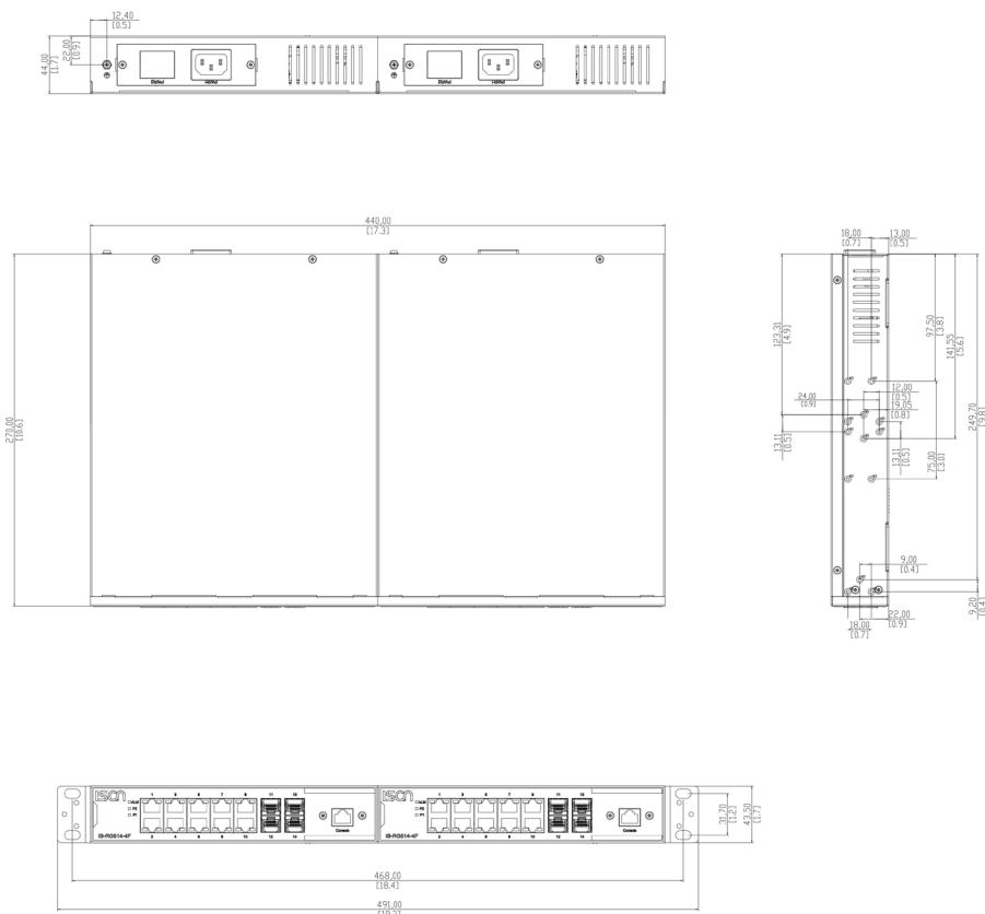
(Twins Mounting)
